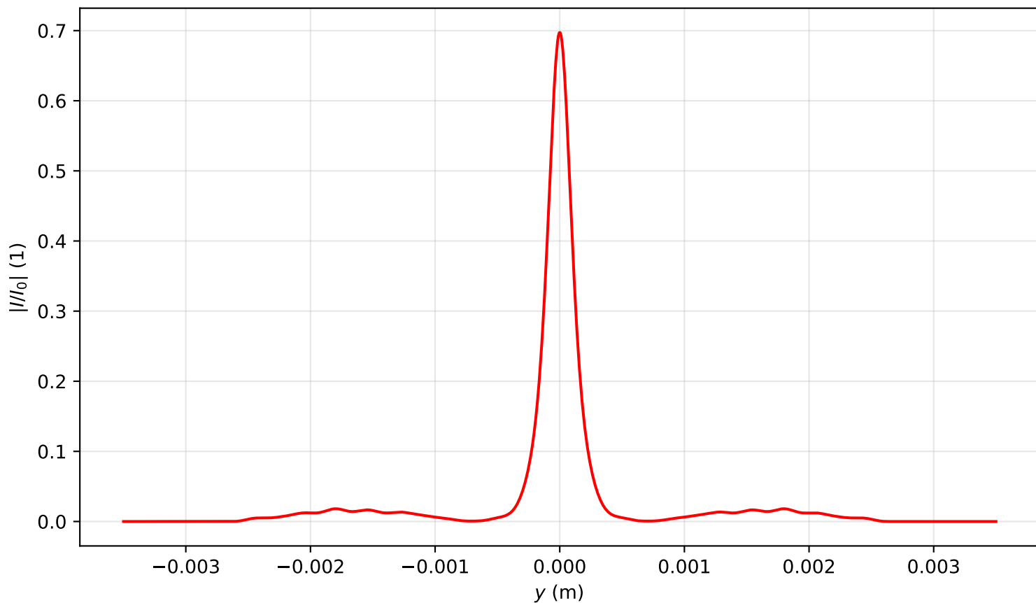
Intensity profile I(x=0, y, z=1.751)/I_0 , P_{in}=9.0P_{cr} , artificial time
